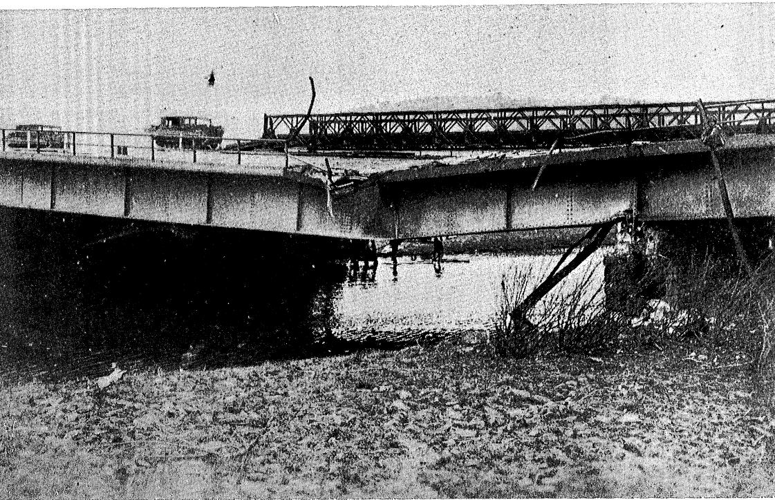
German demolition attempt on the Autobahn—foiled by a Bailey bridge— near Hersfeld.
